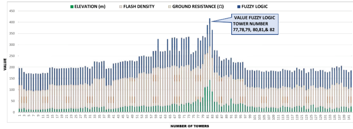
Fig. 6. Fuzzy Logic Result
