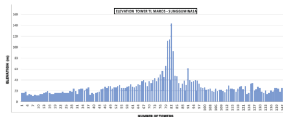
Fig. 2. Elevation of 150 kV Lines Tower
