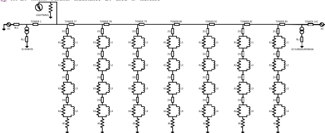
Fig. 9. Modelling of Multistory Tower without TLAs
