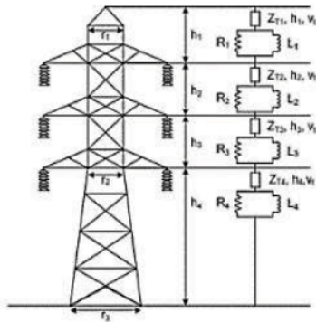
Fig. 7. Model Multistory
