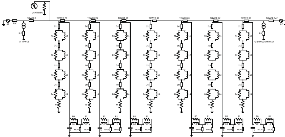
Fig. 10. Modelling of Multistory Tower with 6 TLAs
