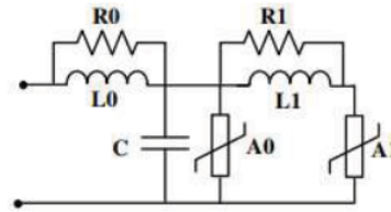
Fig. 8. IEEE Frequency Dependent Model. [18]
