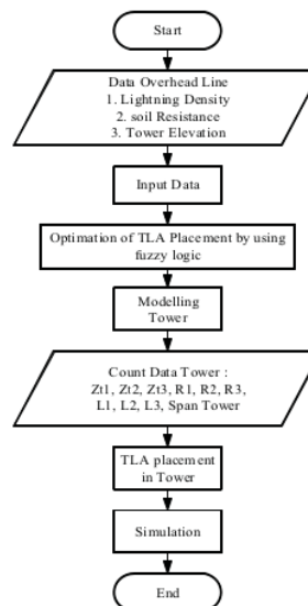
Fig. 5. Placement of TLAs Flowchart.
