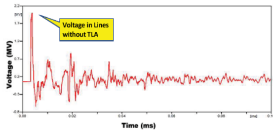
Fig. 11. Result without TLAs placement
